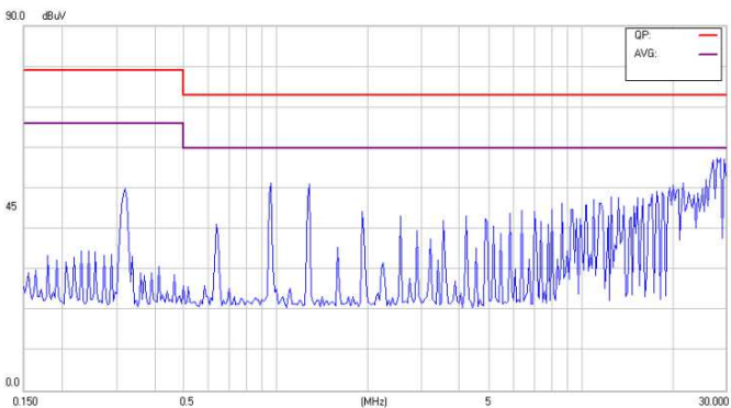
Conducted Class A of CHB350-24S12
