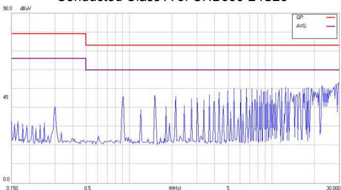
Conducted Class A of CHB350-48S3V3
