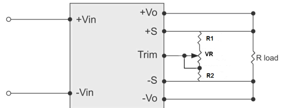
Output voltage trim circuit configuration with VR
