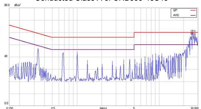
Conducted Class B CHB350-24S12
