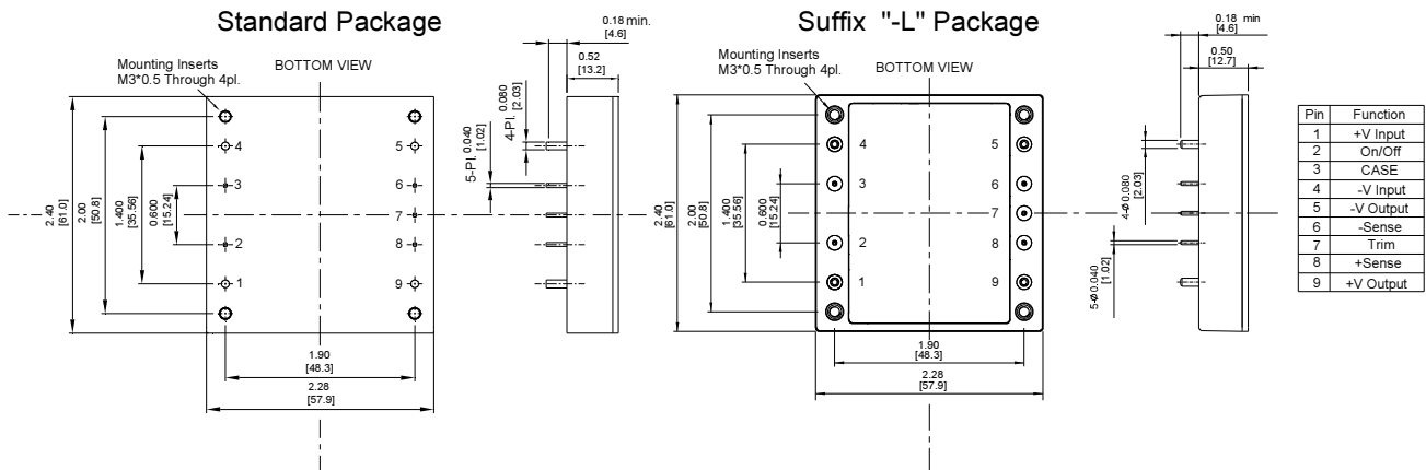
CHB350 Mechanical Outline Diagram
