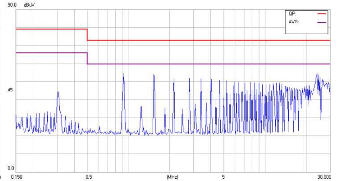
Conducted Class A of CHB350-24S05
