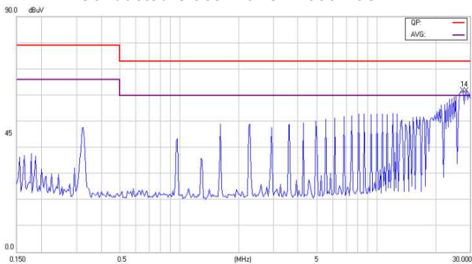
Conducted Class A of CHB350-48S28
