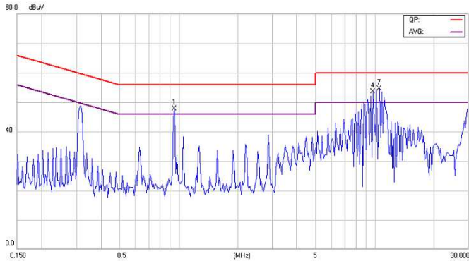
Conducted Class B of CHB350-24S48
