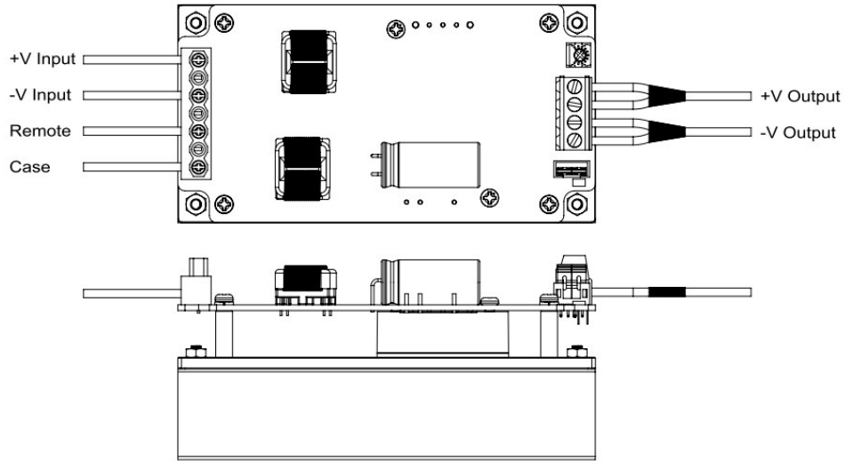
Figures 1 CQB75-300SXX-CMFC with Heat Sink FBL254
