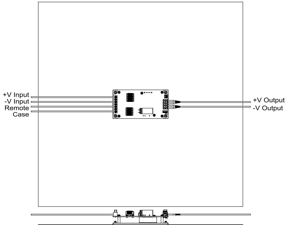
Figures 2 CQB75-300SXX-CMFC with Heat Sink Aluminum Plate (17x17x0.04 inch)
