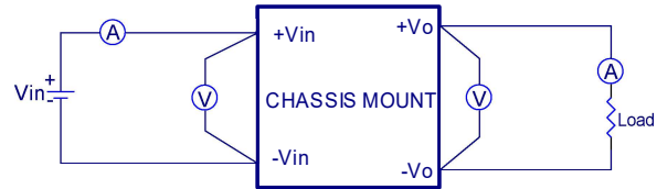
CQB75-300SXX-CMFC(D) Series Test Setup
