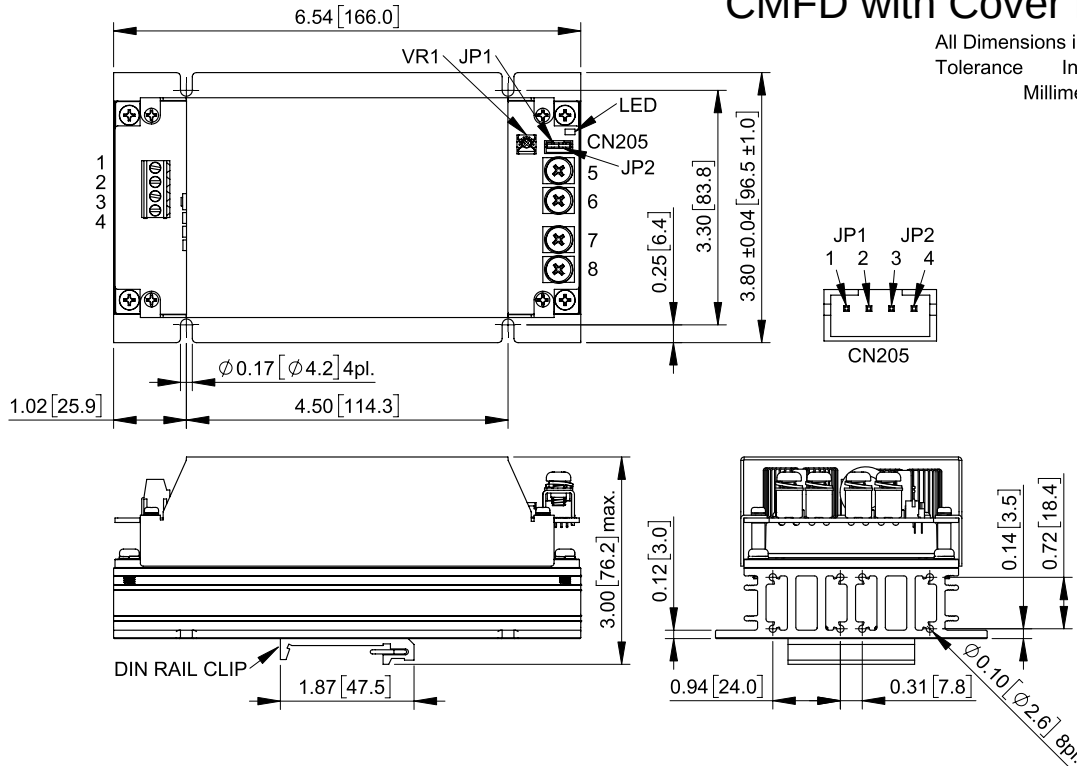
CN205 Pin Connection
