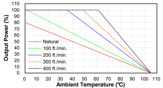
CQB100W18-36S12 Derating Curve without Heatsink (Vin=36V)
