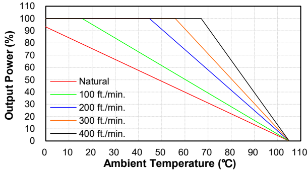
CQB100W8-36S05, 15, 24 Derating Curve without Heatsink (Vin=36V)
