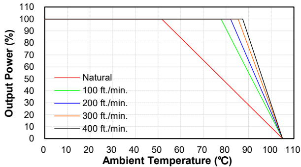
CQB100W8-36S05, 15, 24 Derating Curve with Heatsink QBT210 (Vin=36V)
