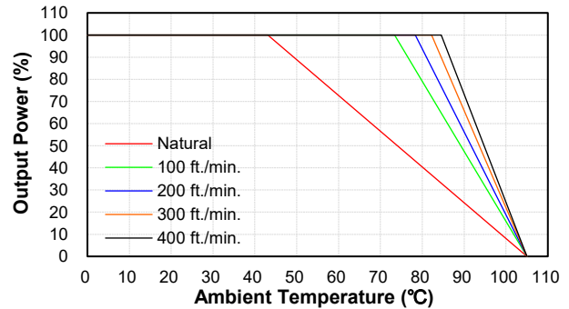
CQB100W8-36S12 Derating Curve with Heatsink QBT210 (Vin=36V)
