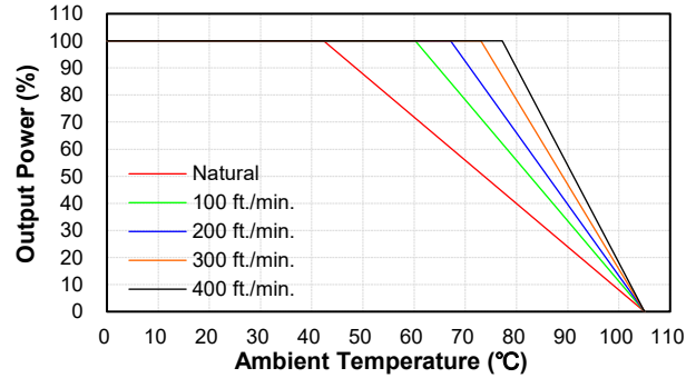
CQB100W8-36S05, 15, 24 Derating Curve with Heatsink QBL127 (Vin=36V)
