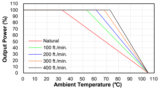
CQB100W8-36S12 Derating Curve with Heatsink QBL127 (Vin=36V)
