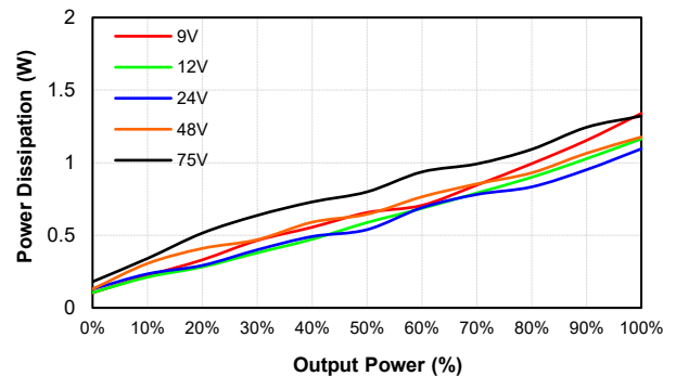
EC4SAW8-48D05N Pd Vs Po @25 Deg. C
