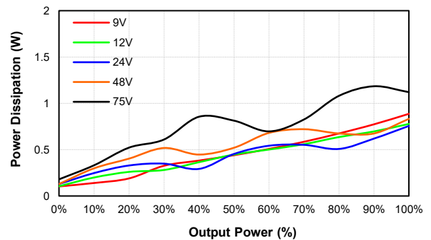
EC4SAW8-48S15N Pd Vs Po @25 Deg. C
