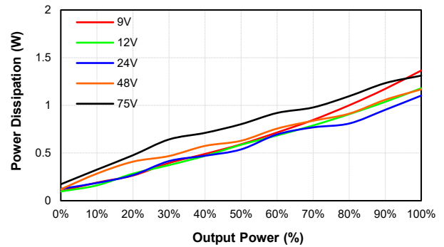
EC4SAW8-48S05N Pd Vs Po @25 Deg. C
