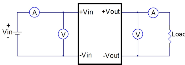
EC2SAW8 Series Test Setup
