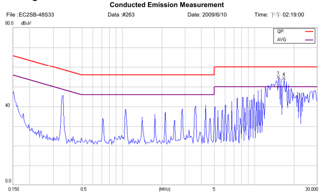
Figure 36 Conducted Class B of EC2SB-48S33
