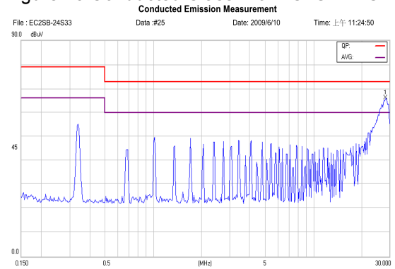
Figure 20 Conducted Class A of EC2SB-24S33
