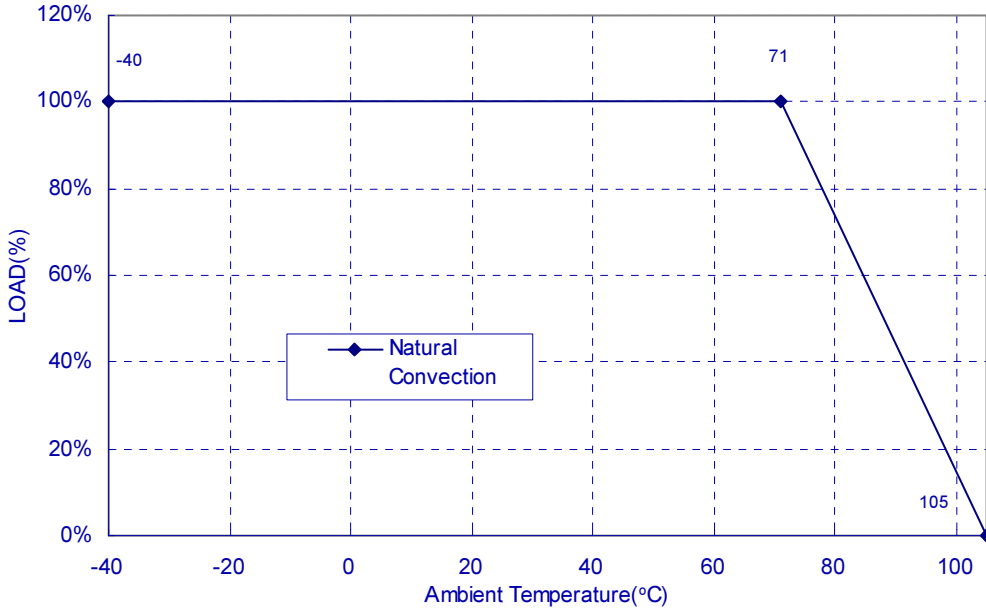
Typical Derating curve for Natural Convection
