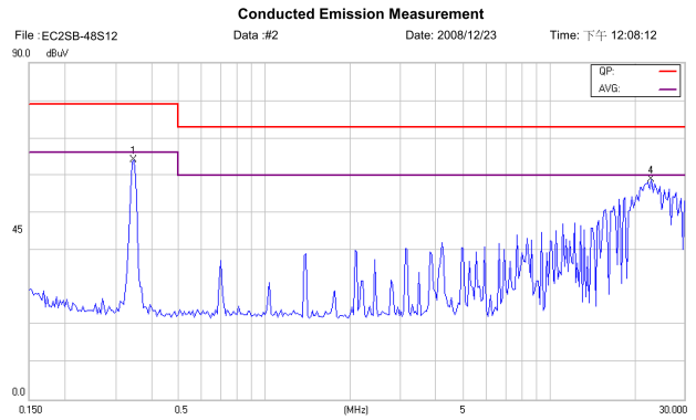
Figure 26 Conducted Class A of EC2SB-48S12
