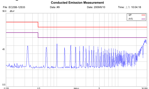
Figure 16 Conducted Class A of EC2SB-12S33
