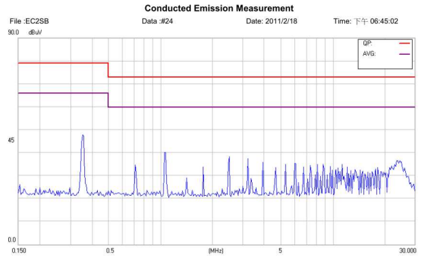
Figure 14 Conducted Class A of EC2SB-05D12
