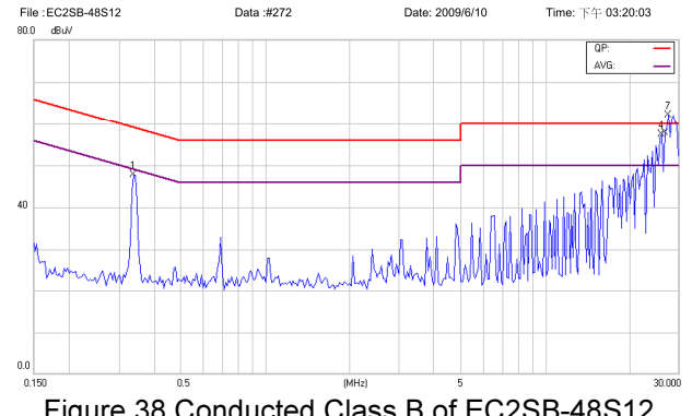
Figure 38 Conducted Class B of EC2SB-48S12
