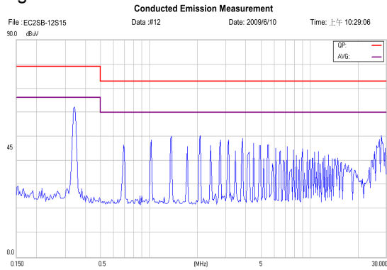
Figure 19 Conducted Class A of EC2SB-12S15
