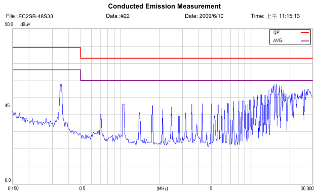
Figure 24 Conducted Class A of EC2SB-48S33
