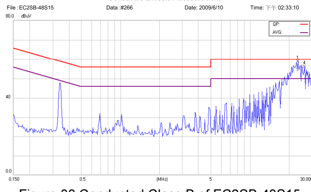
Figure 38 Conducted Class B of EC2SB-48S15
