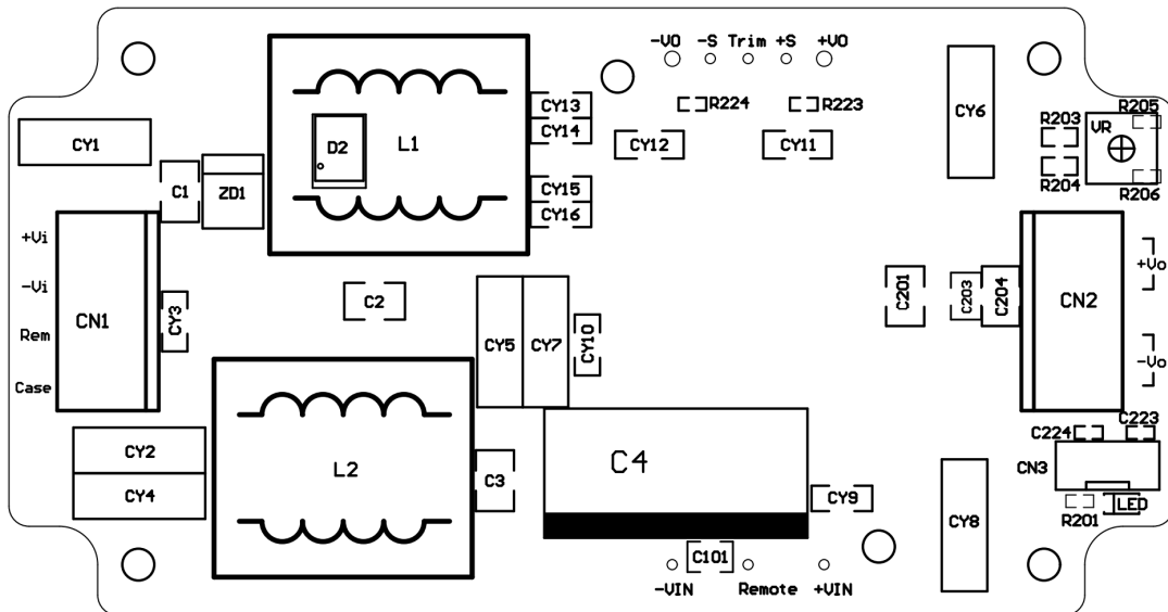
Figure2 Component Placement
